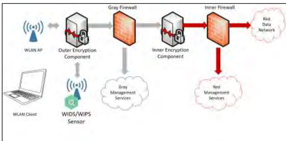
Figure 1: WLAN with Integrated Gray WIDS/WIPS
