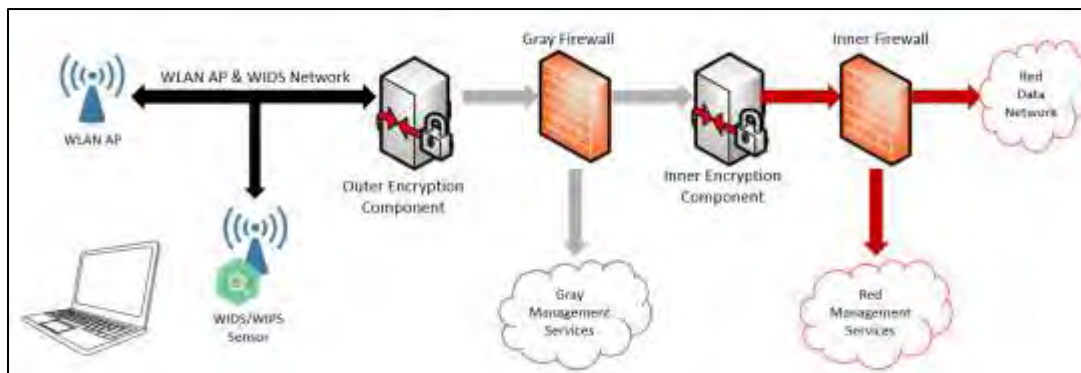
Figure 7: WLAN with Integrated WIDS/WIPS Single Network
