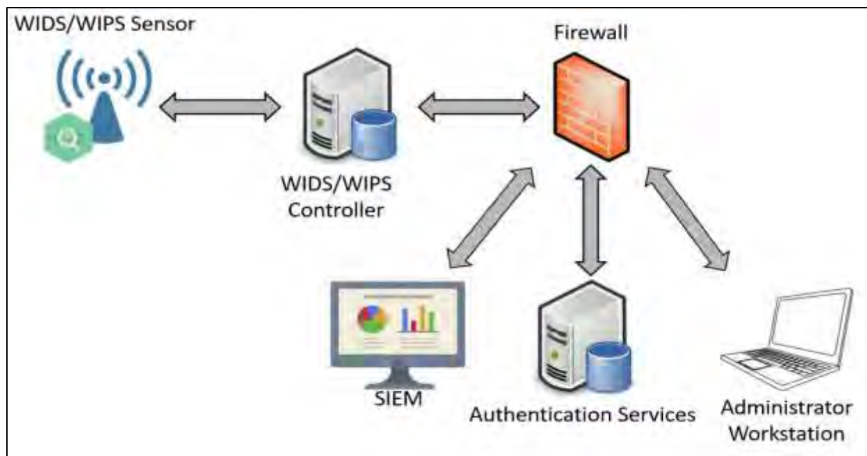
Figure 9: WIDS/WIPS Components
