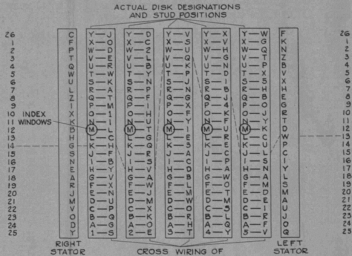
FIG. 17 CROSS WIRING OF INDIVIDUAL DISKS CIPHER DISK CONNECTION
